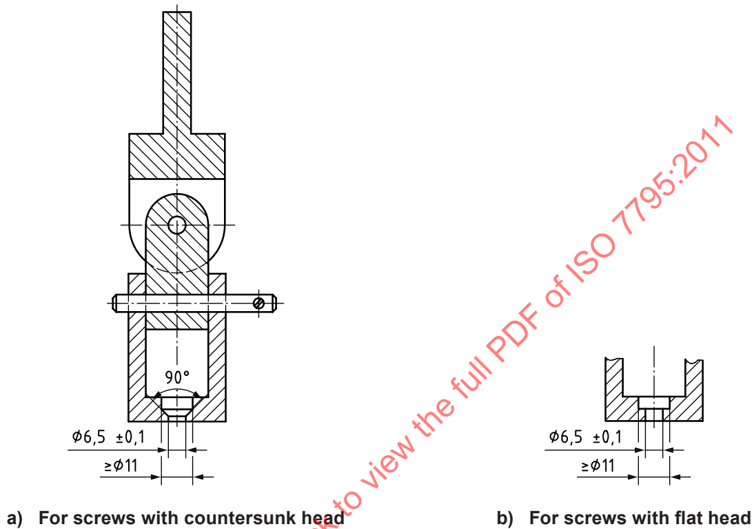
Figure 3 — Pull-out apparatus
