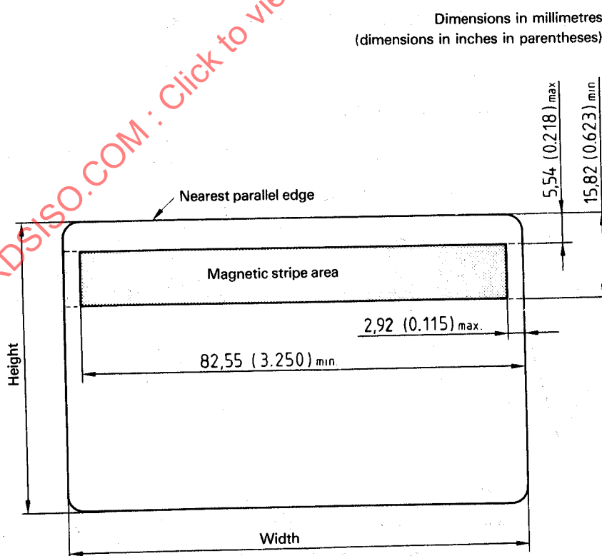
Figure 2 — Location of magnetic material for tracks 1, 2 and 3 on ID-1 type card
