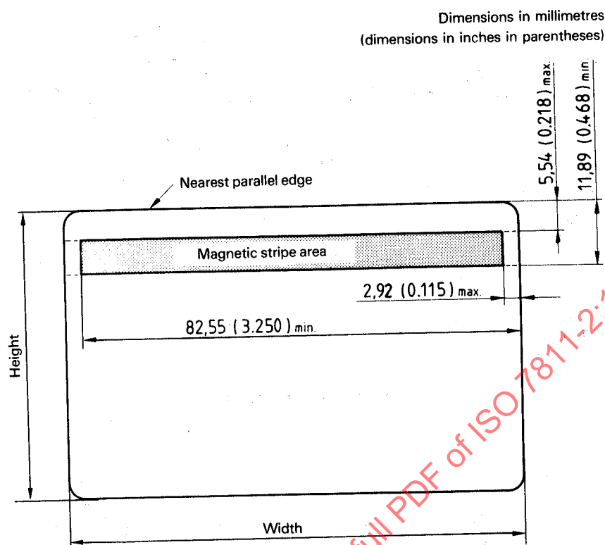
Figure 1 — Location of magnetic material for tracks 1 and 2 only on ID-1 type card
