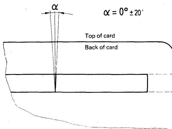
Figure 7 — Angle of recording
