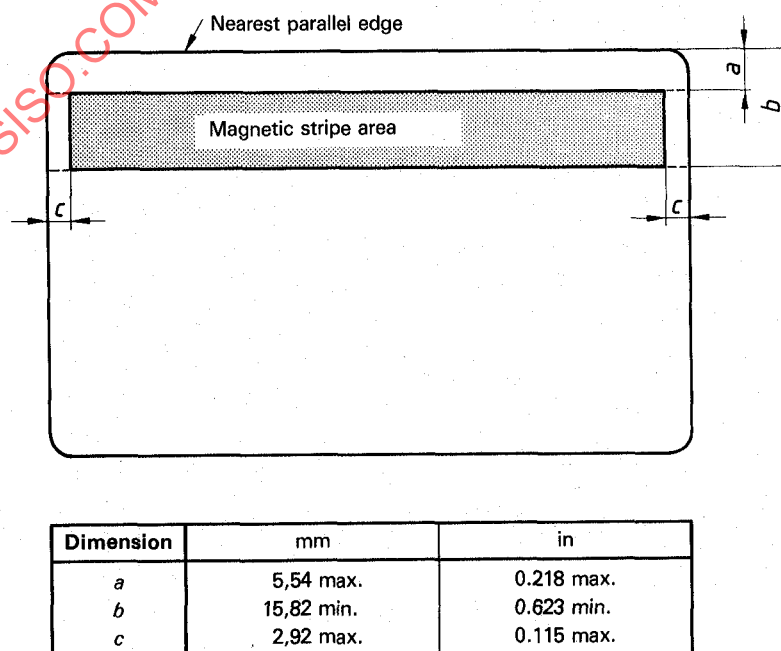
Figure 1 — Location of magnetic stripe area for track 3
