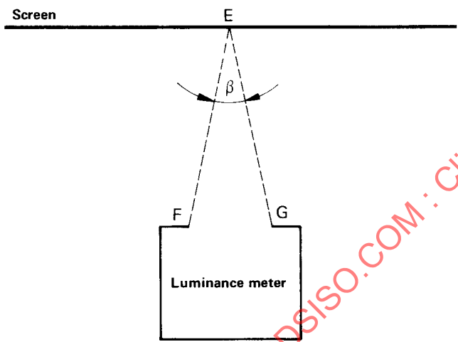
FIGURE 1 — Diagram showing the definition of the angle of acceptance
