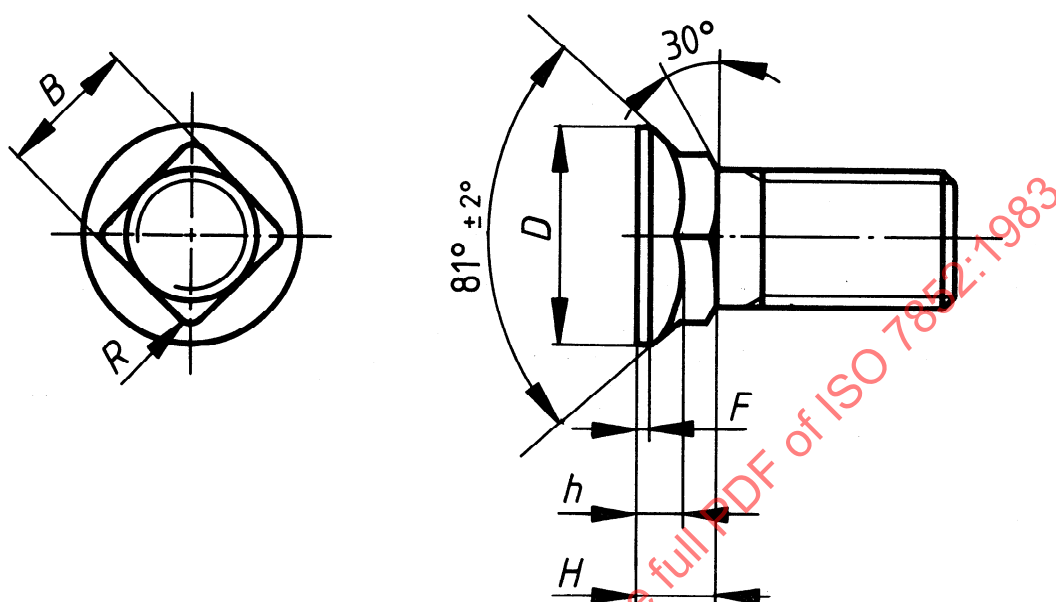
Figure 1 — Shapes and dimensions of plough bolt heads
