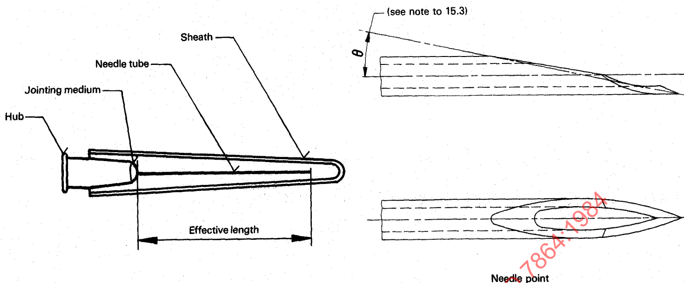
Figure — Typical hypodermic needle for single use
