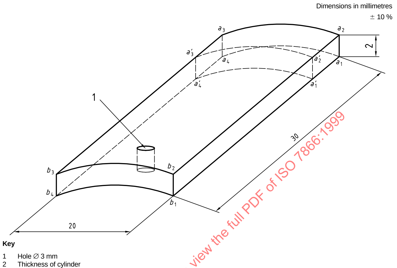
Figure A.2 — Specimen shape and dimensions
