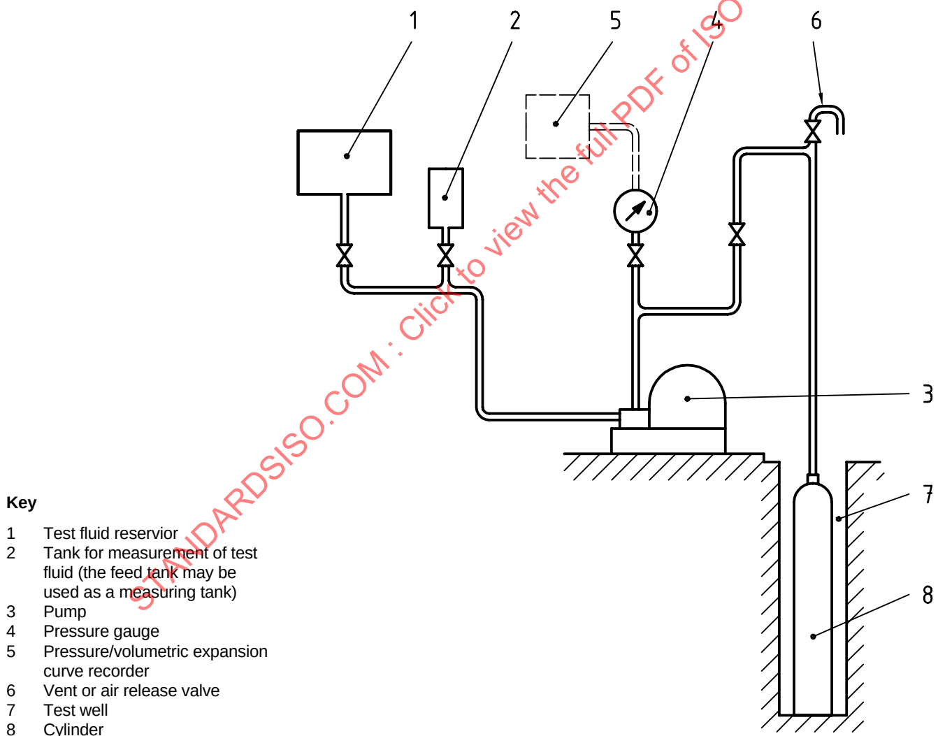
Figure 6 — Typical hydraulic bursting test installation
