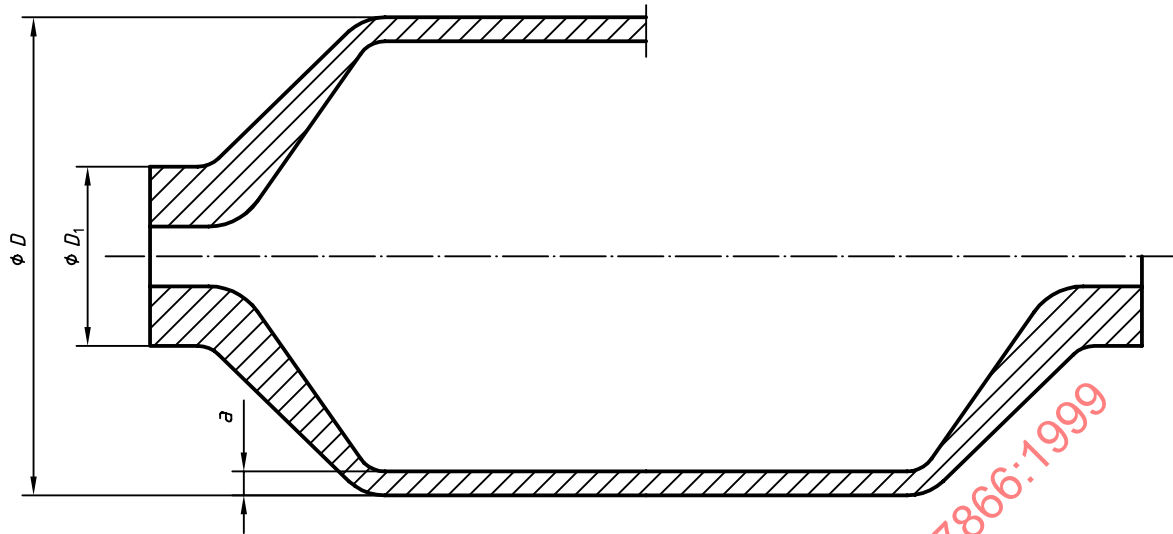
Figure 2 — Necked ends from tube
