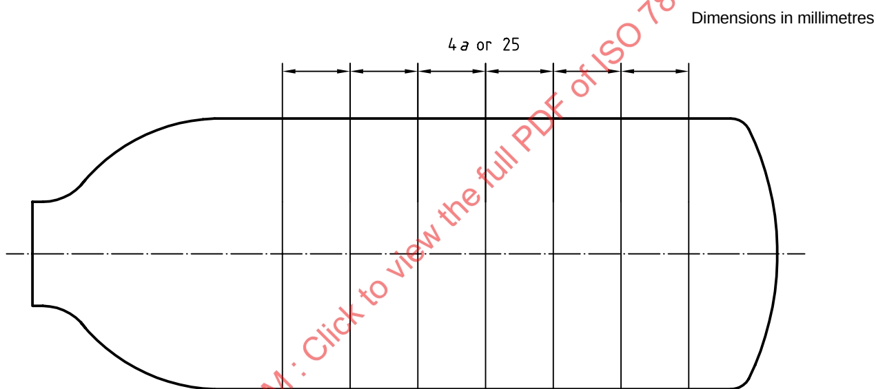
Figure A.4 — Specimen ring locations
