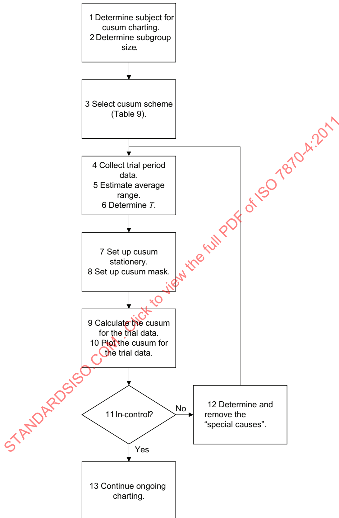
Figure 12 — Cusum set-up protocol
