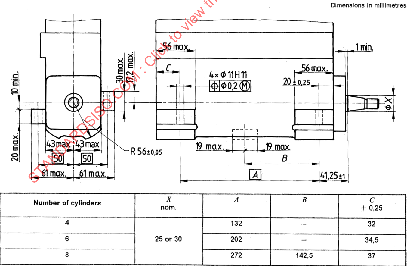
Figure 1 — Cradle-mounted in-line fuel injection pump — Type 1
