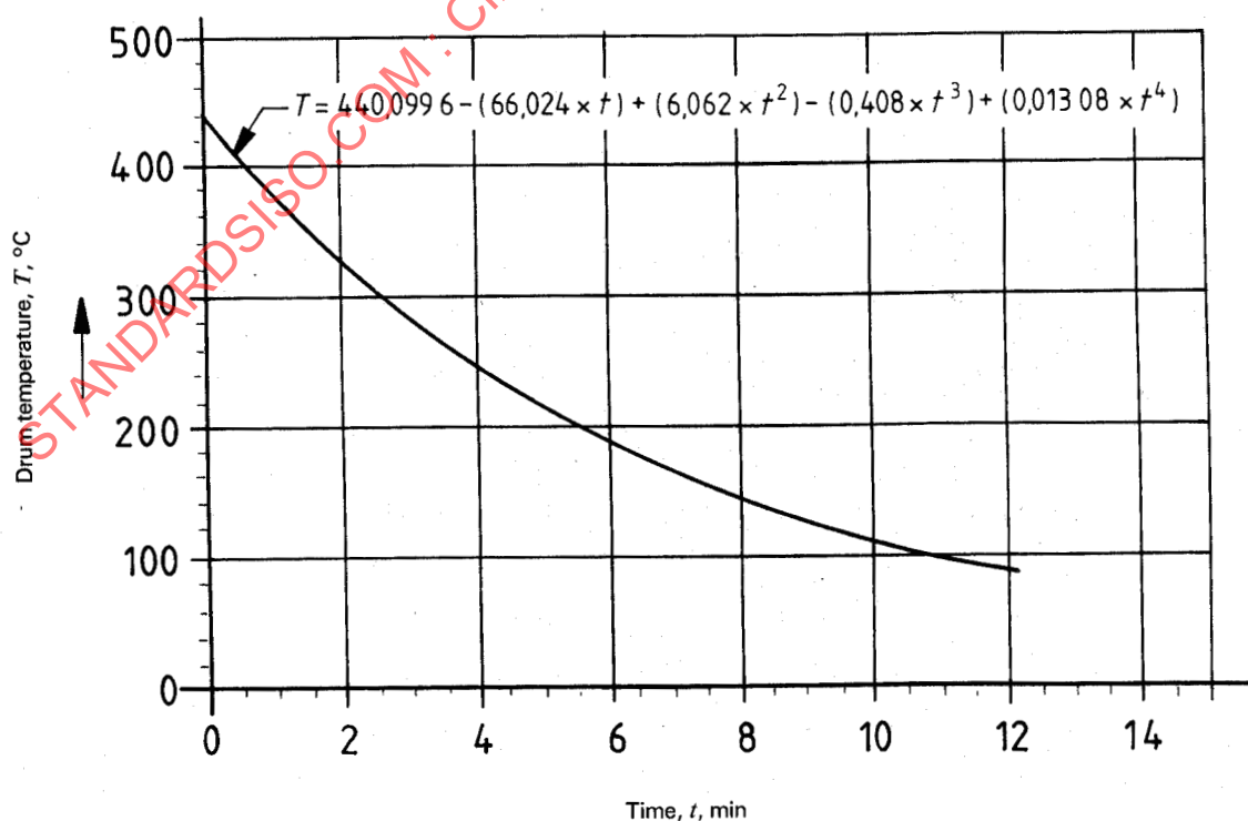
Figure 4 — Temperature/time graph for drum cooling
