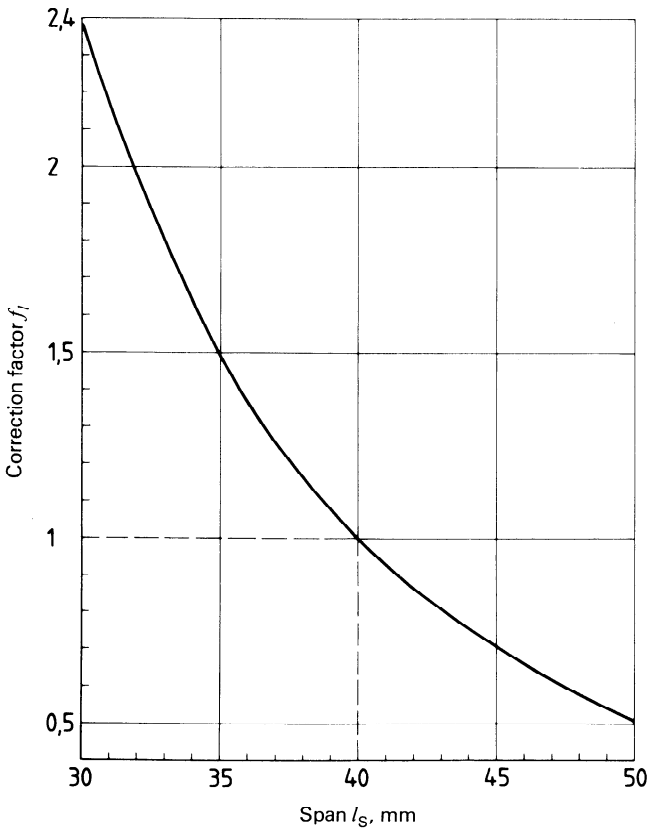
Figure 3 — Correction factor f_l for the estimation of the time interval \Delta t'_1 according to equation (9), taking into account spans l_s other than that given in table 1
