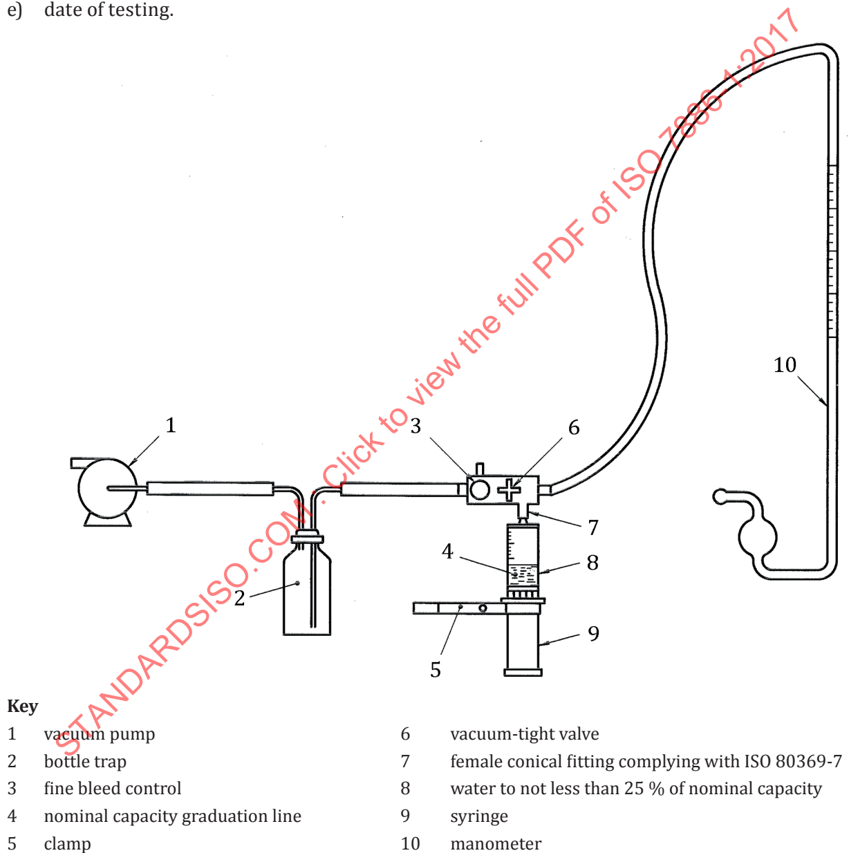
Figure B.1 — Apparatus for aspiration test
