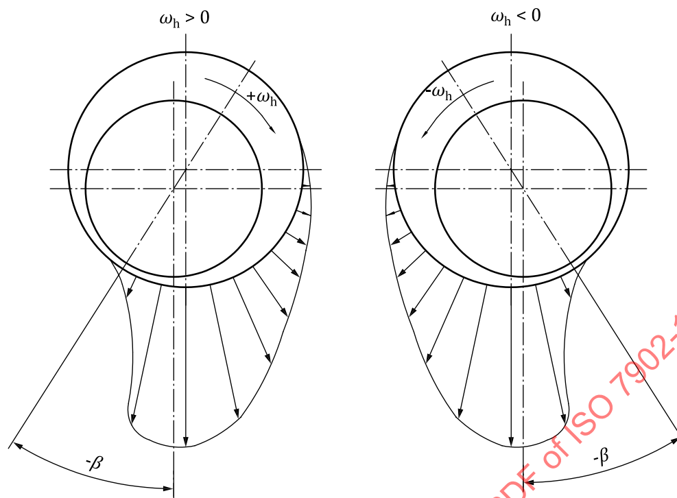
Figure 4 — Definition of the attitude angle \beta
