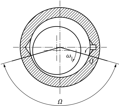
Figure A.2 — Partial bearing lubricated via pocket
