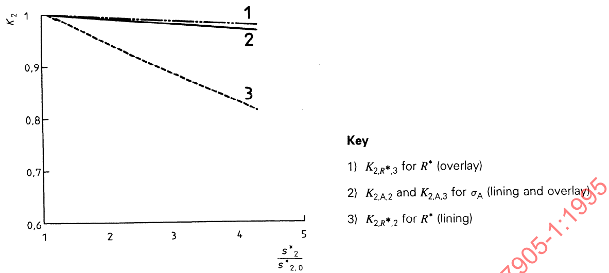
Figure A.6 — Correction factor for lining thickness
