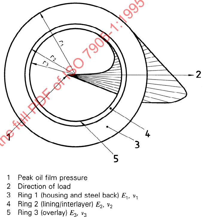
Figure A.1 — Bearing ring model
