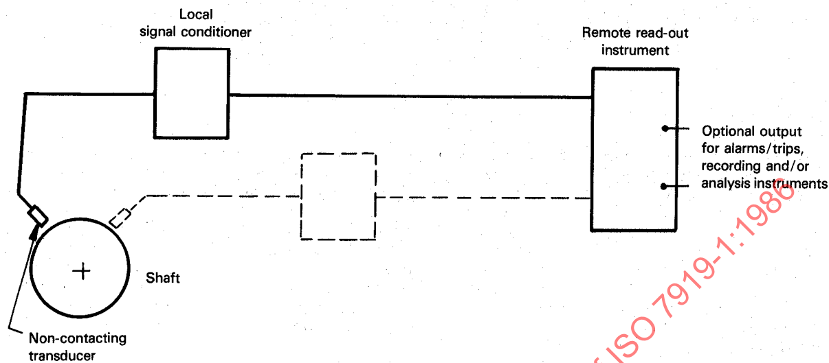
Figure 3 — Schematic diagram of relative motion measurement system using non-contacting transducers (see clause B.1)
