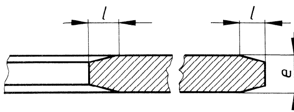
Figure 3 — Disk, edge chamfers, cross-sectional view
