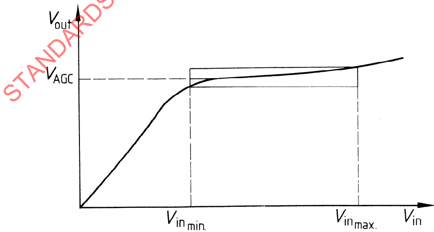
Figure 5 — AGC-amplifier characteristics
