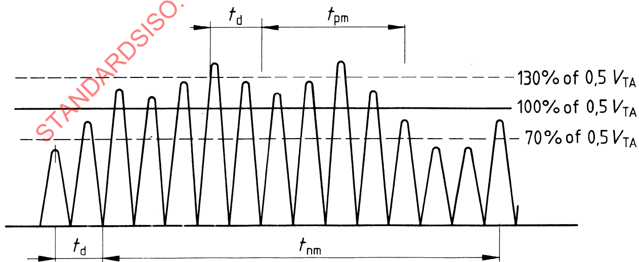
Figure 7 — Modulation tests
