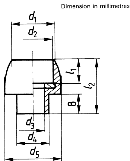
Figure 2 — Insulation bush
