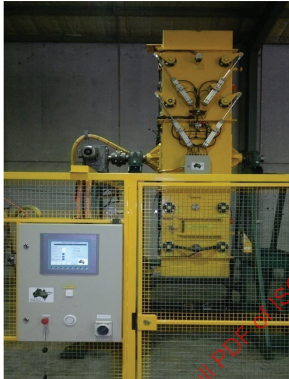
Figure A.2 — Example of automatic drop shatter machine
