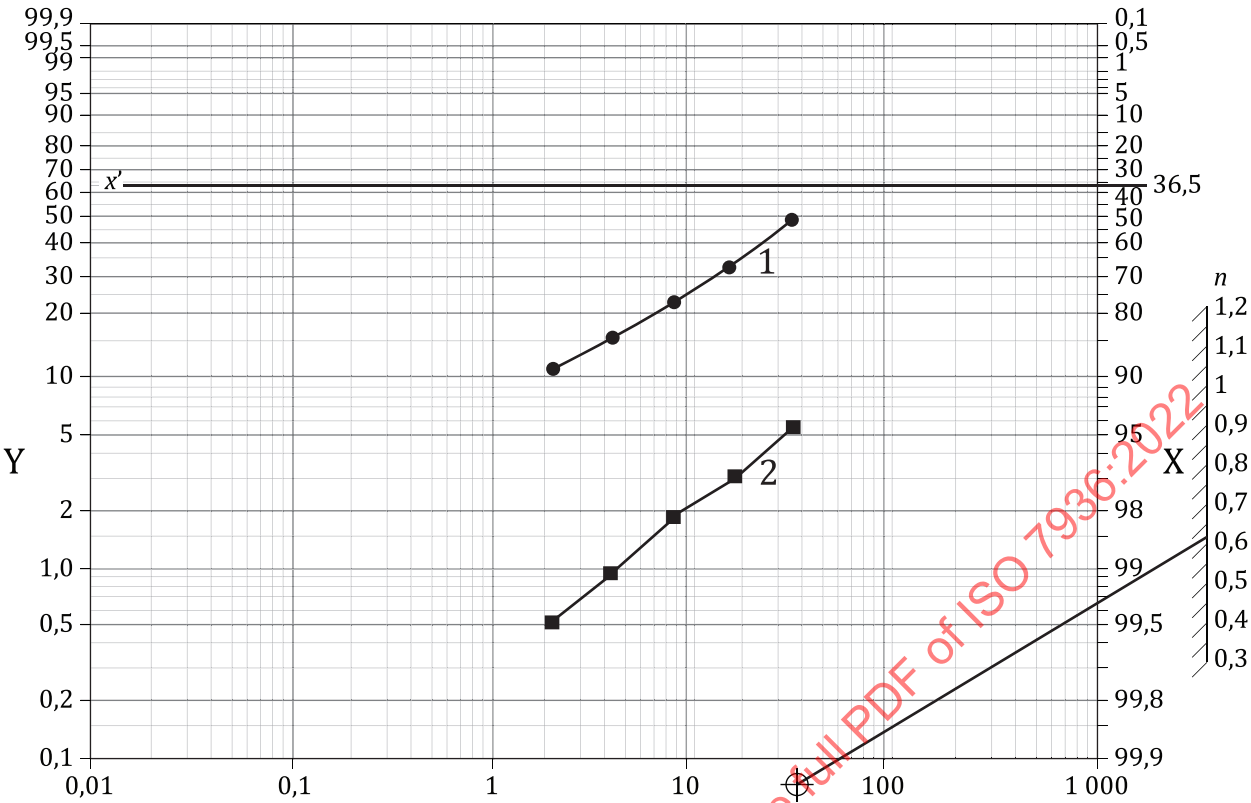
Figure A.5 — Rosin Rammler plot of size distribution before and after drop shatter
