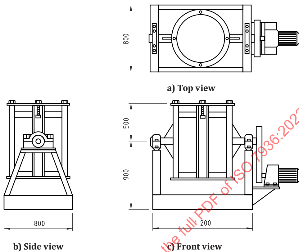
Figure B.1 — Typical drum tumbler
