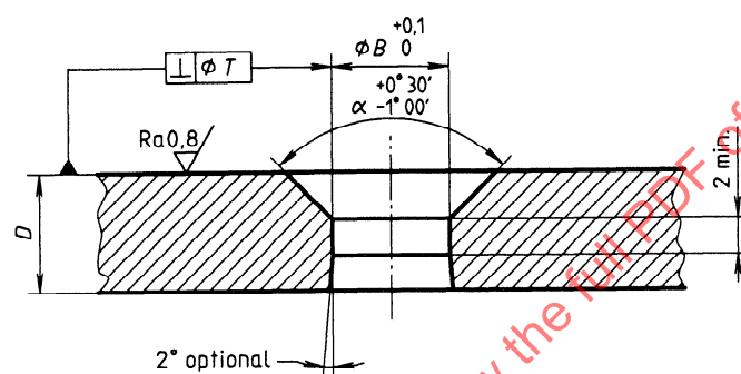
Upper cup for flush head bolts
