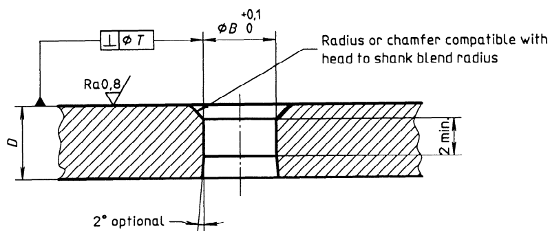
Upper cup for protruding head bolts
