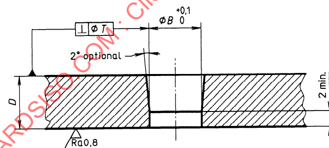
Lower cup
