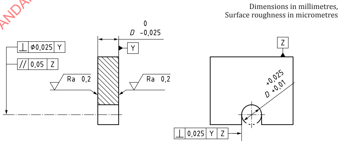
Figure 4 — Double shear test — Test device
