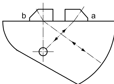
Figure 5 — Miniature angle-beam probes — Sensitivity setting
