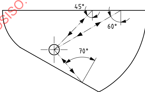
Figure 7 — Miniature angle-beam probes — Determination of beam angle
