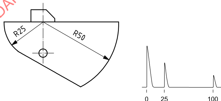
a) For a range of 125 mm
