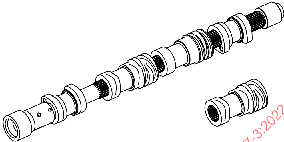
Figure 3 — Assembled camshaft
