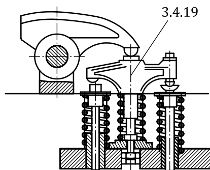
Figure 22 — Valve bridge
