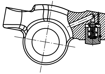
Figure 25 — Exhaust valve brake rocker arm
