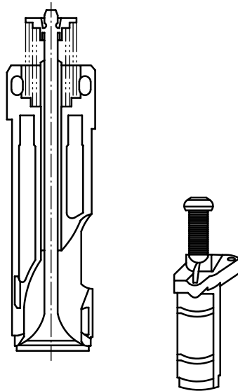
Figure 13 — Valve cage
