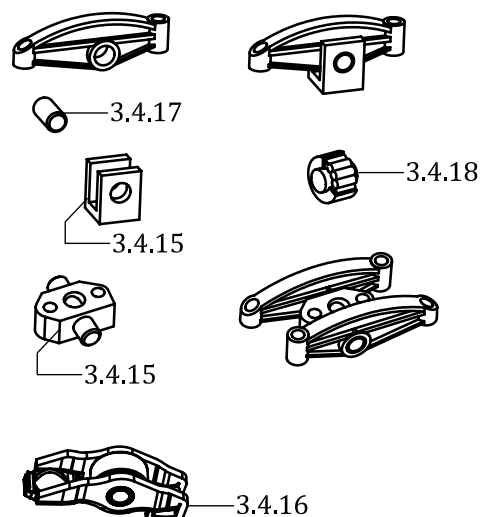
Figure 21 — Rocker arm bracket group
