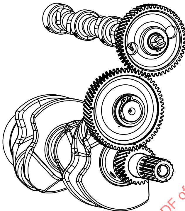
Figure 5 — Gear drive
