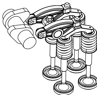
Figure 27 — Single overhead camshaft
