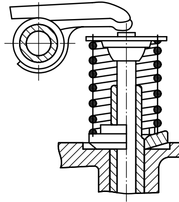
Figure 23 — Valve rotator
