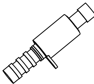
Figure 11 — Control valve for variable valve timing mechanism
