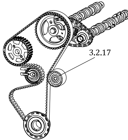
Figure 9 — Idler assembly
