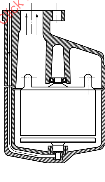
Figure 21 — Rotor drum
