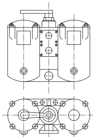
Figure 10 — Duplex lubricating oil filter
