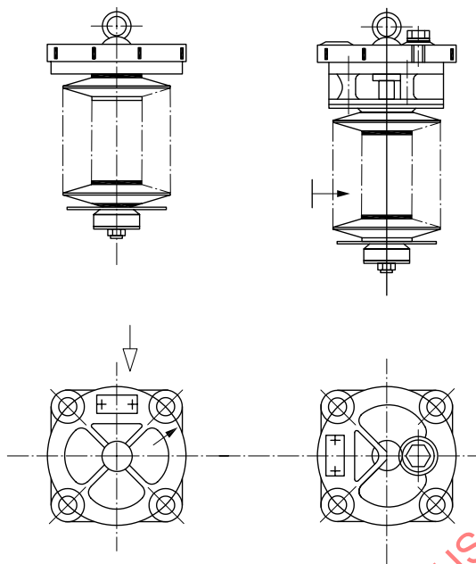
Figure 20 — Filter insert
