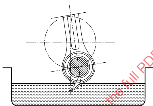
Figure 1 — Dip lubrication
