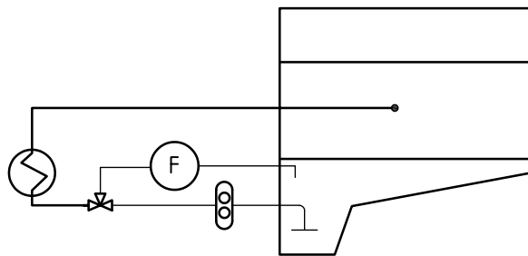
Figure 8 — Bypass lubricating oil filter
