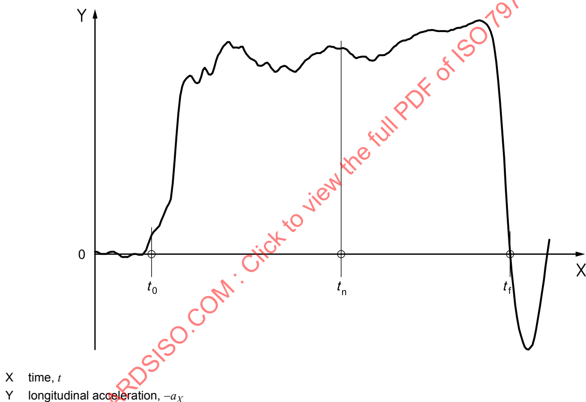
Figure 2 — Longitudinal acceleration, -a_X , versus time
