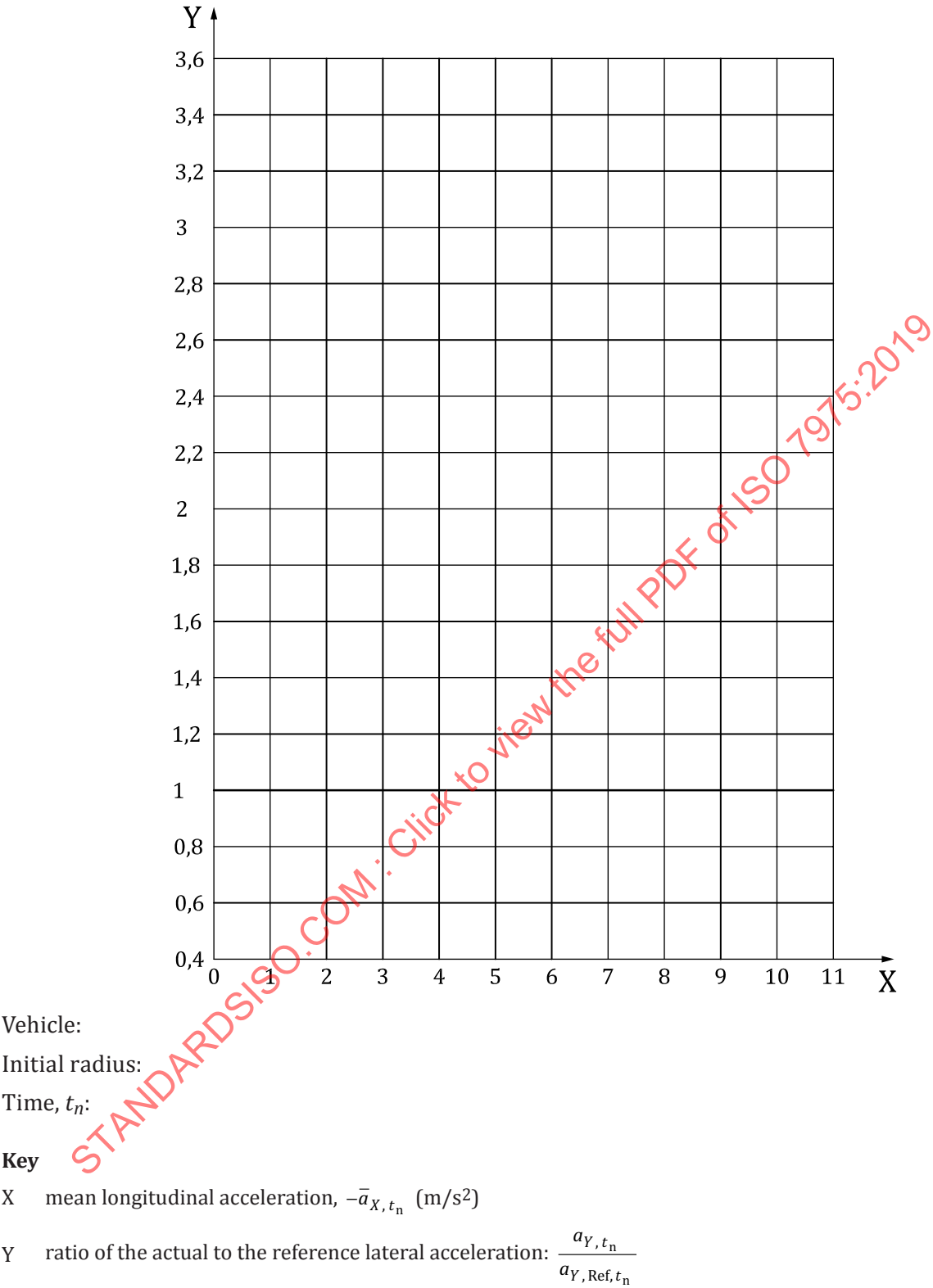
Figure A.6 — The ratio of the value of the lateral acceleration, a_{Y,t_n} , at time t_n to the reference value of the lateral acceleration, a_{Y,Ref,t_n} , at actual time t_n , as a function of the mean longitudinal acceleration, -\bar{a}_{X,t_n}
