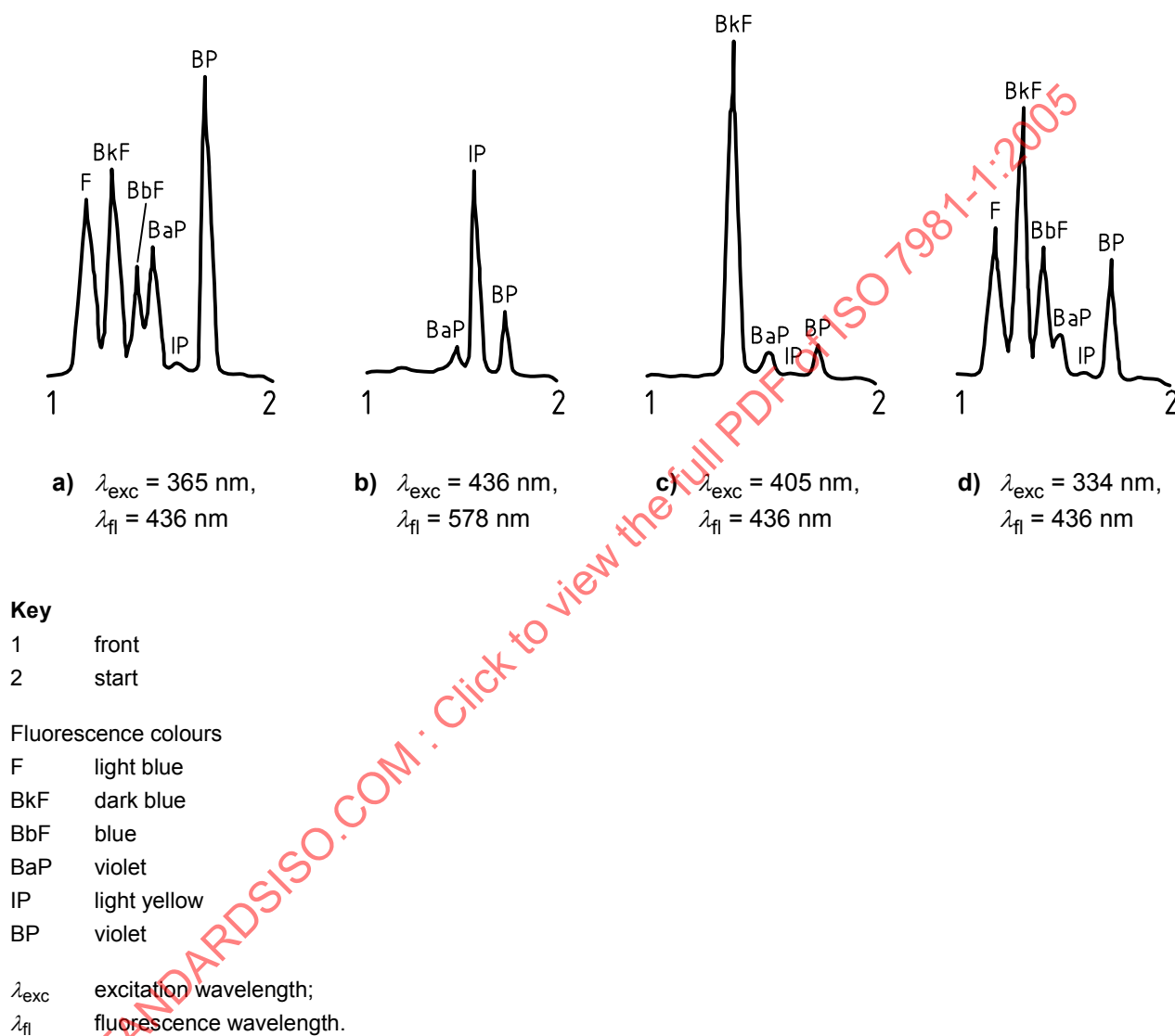
Figure B.1 — Selective detection of the six PAH
