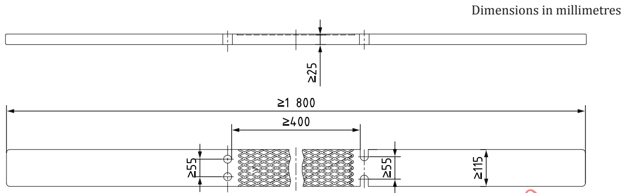
Figure 3 — Pilot ladder spreader step and replacement spreader step construction, hole and slot types for side ropes
