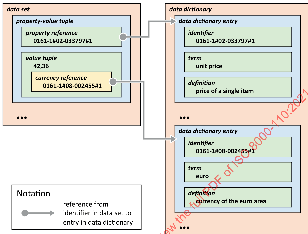
Figure 7 — Representing a currency amount by referencing the currency in the data dictionary
