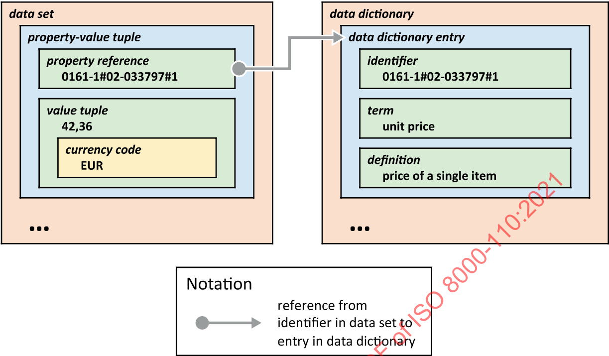
Figure 8 — Representing a currency amount by a currency code
