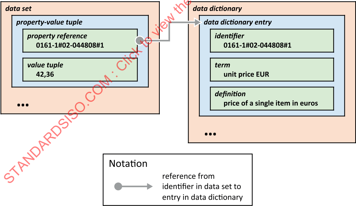
Figure 9 — Representing a currency amount by including the currency in the property definition
