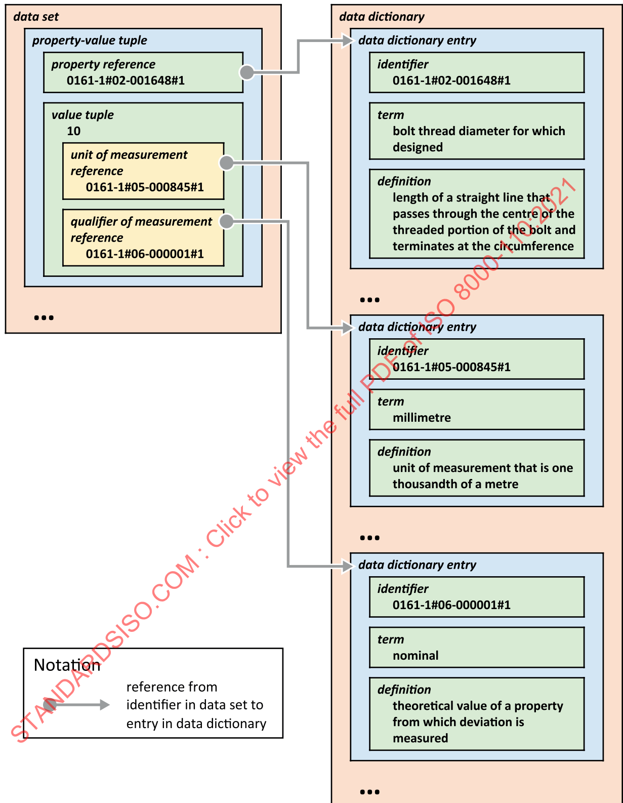
Figure 4 — Representing a quantity by referencing the unit of measurement and qualifier in the data dictionary
