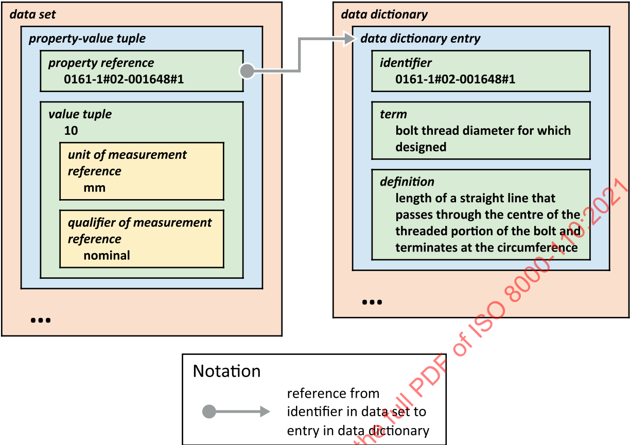
Figure 5 — Representing a quantity by symbols for the unit of measurement and qualifier
