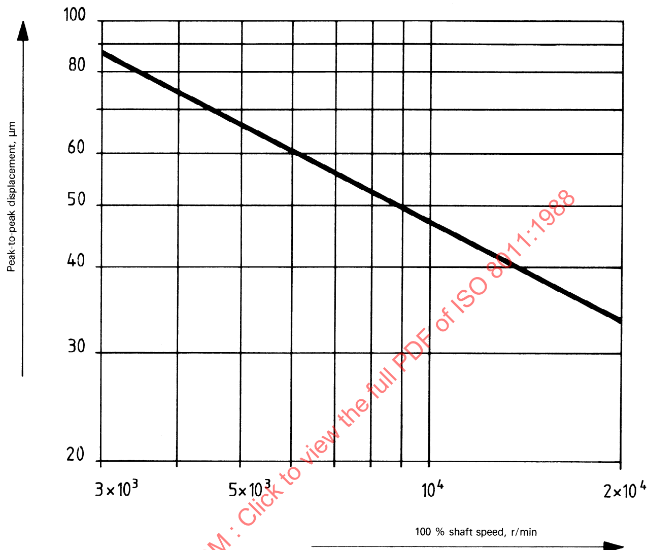
Figure 5 — Guideline to the order of magnitude of the permissible maximum shaft movement
