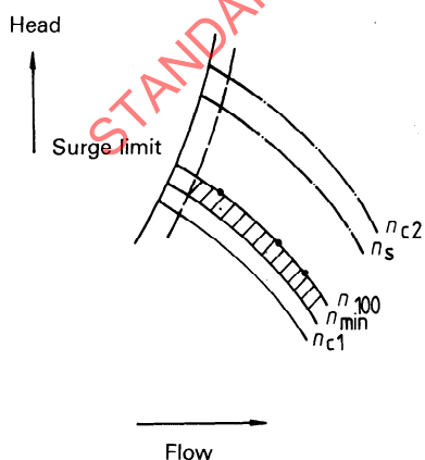
Figure 1 — Illustration of various definitions in terms of a) a single-shaft turbine or expander drive, b) all drives involving a split-shaft gas turbine and c) an electric motor drive
