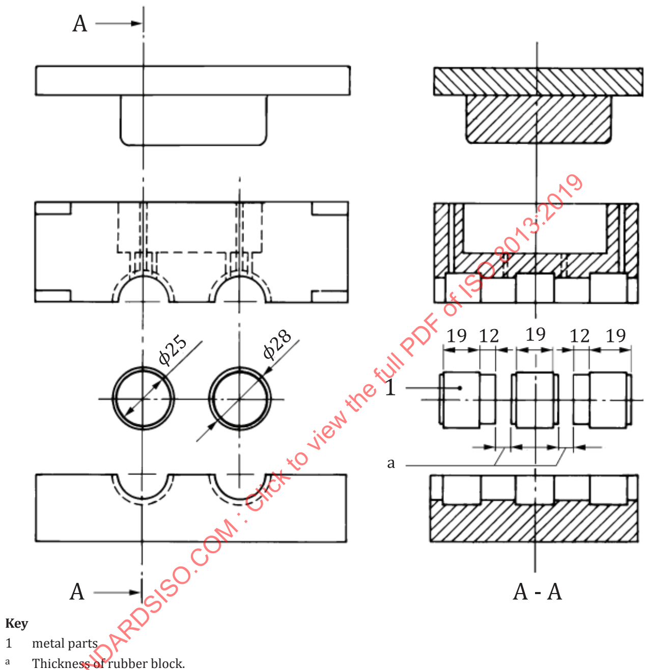
Figure 5 — Mould for double-shear test piece
