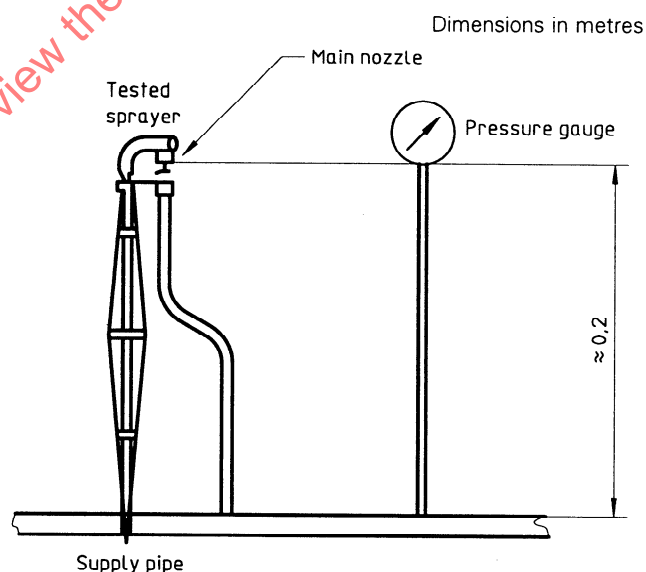
Figure 1 — Measurement of sprayer pressure
