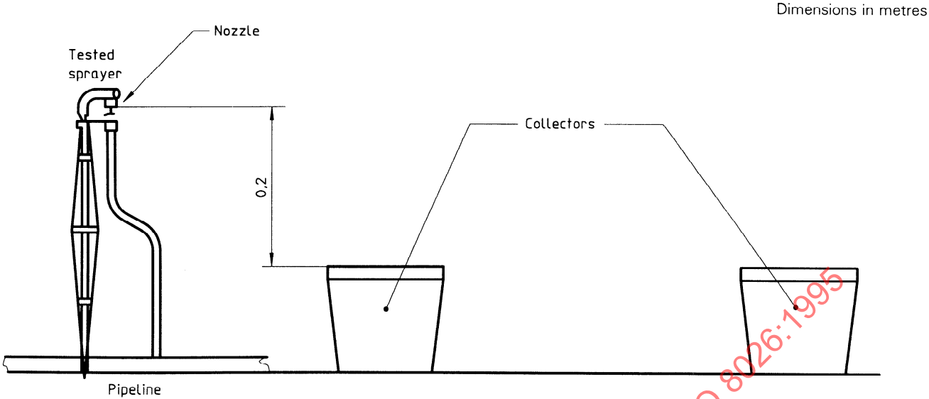
Figure 4 — Sprayer arrangement for water distribution test
