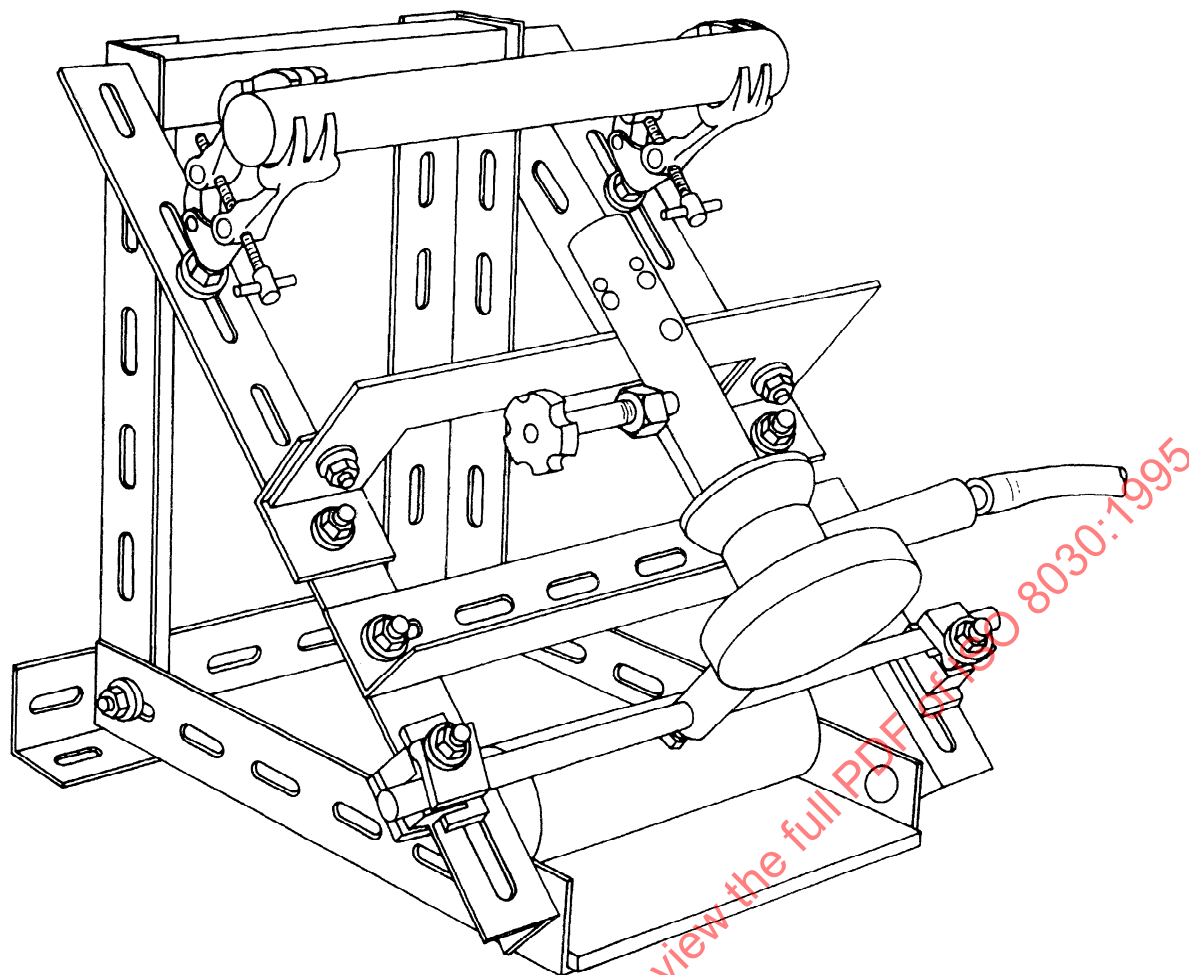
Figure 2 — Arrangement for flammability test
