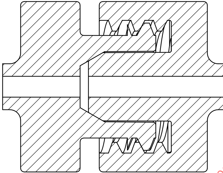
Figure B.5 — R1 small-bore connector assembly
