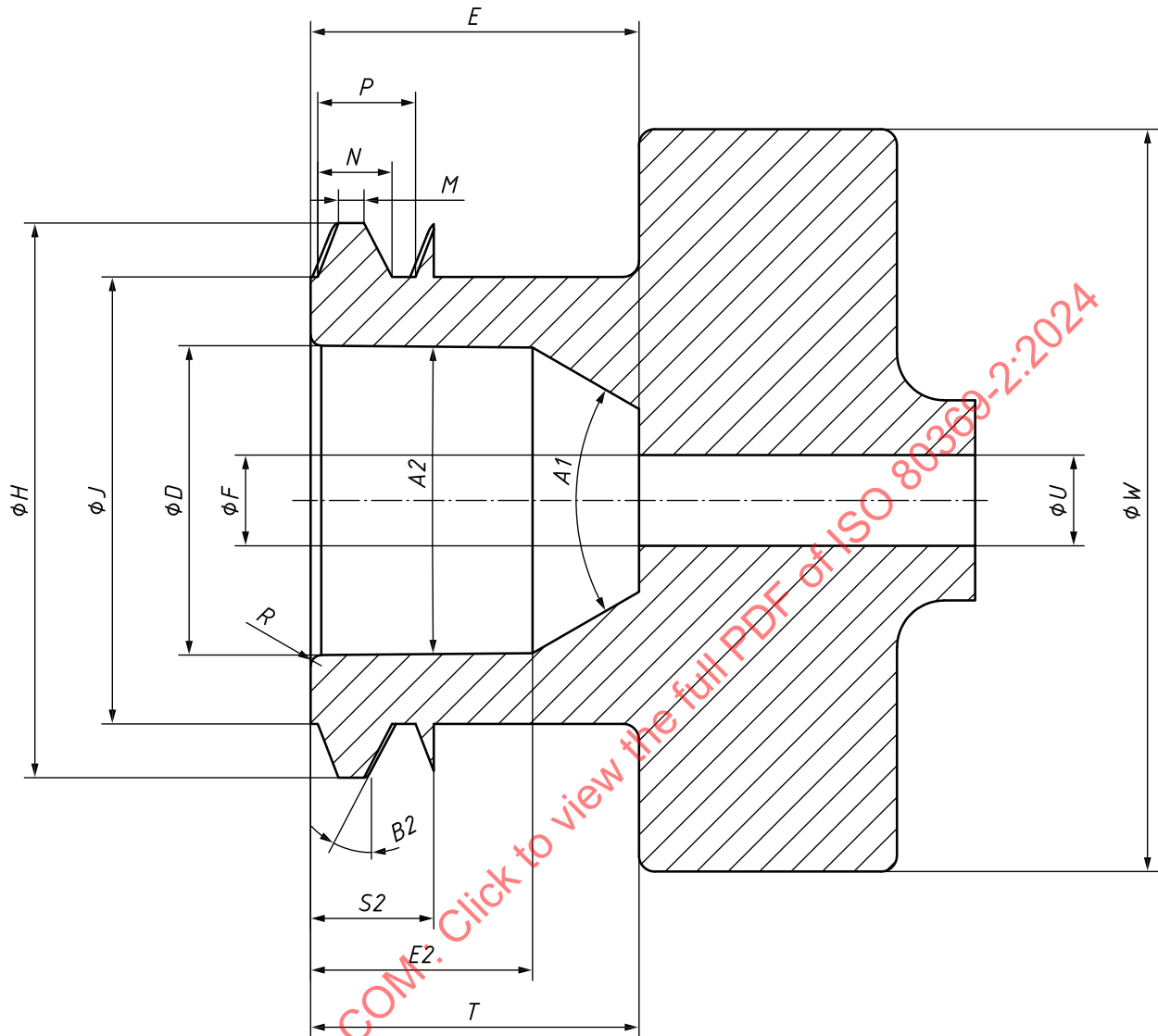
Figure B.2 — R1 socket small-bore connector
