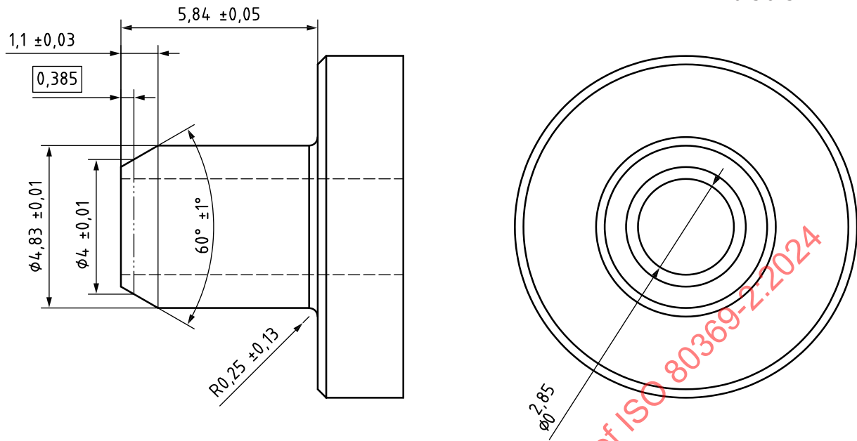
Figure C.5 — Cone reference connector cone taper insert for testing R1 socket connectors for leakage, separation from unscrewing, separation from axial load and resistance to overriding, stress cracking and non-interconnectable characteristics
