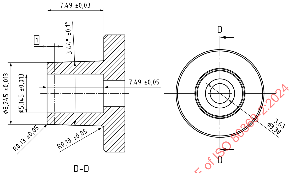
Figure C.12 — Cone reference connector cone taper insert for testing R2 socket connectors for leakage, separation from unscrewing, stress cracking and separation from axial load and resistance to overriding
