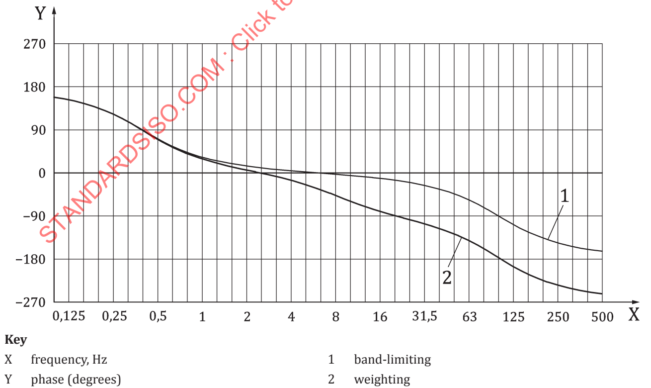
Figure B.4 — Phase of frequency weighting W_c for horizontal whole-body vibration, x-axis, seat back, seated person, based on ISO 2631-1
