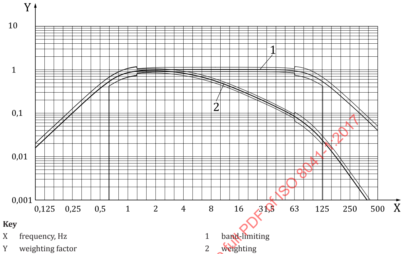
Figure B.17 — Magnitude of frequency weighting W_m for whole-body vibration in buildings, all directions, based on ISO 2631-2
