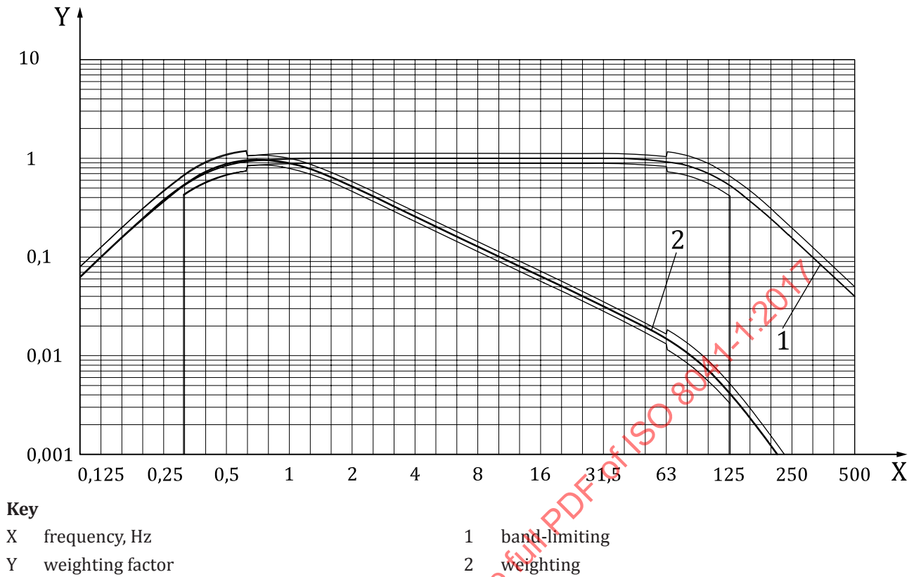
Figure B.7 — Magnitude of frequency weighting W_e for rotational whole-body vibration, all directions, seated person, based on ISO 2631-1
