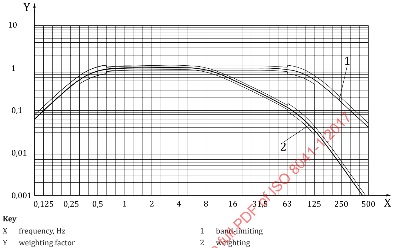
Figure B.3 — Magnitude of frequency weighting W_c for horizontal whole-body vibration, x-axis, seat back, seated person, based on ISO 2631-1
