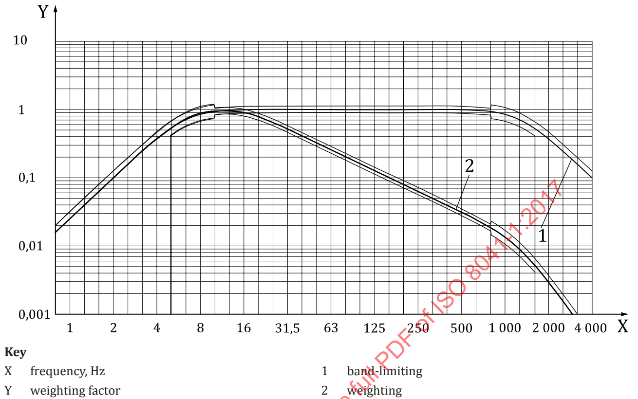
Figure B.11 — Magnitude of frequency weighting W_h for hand-arm vibration, all directions, based on ISO 5349-1
