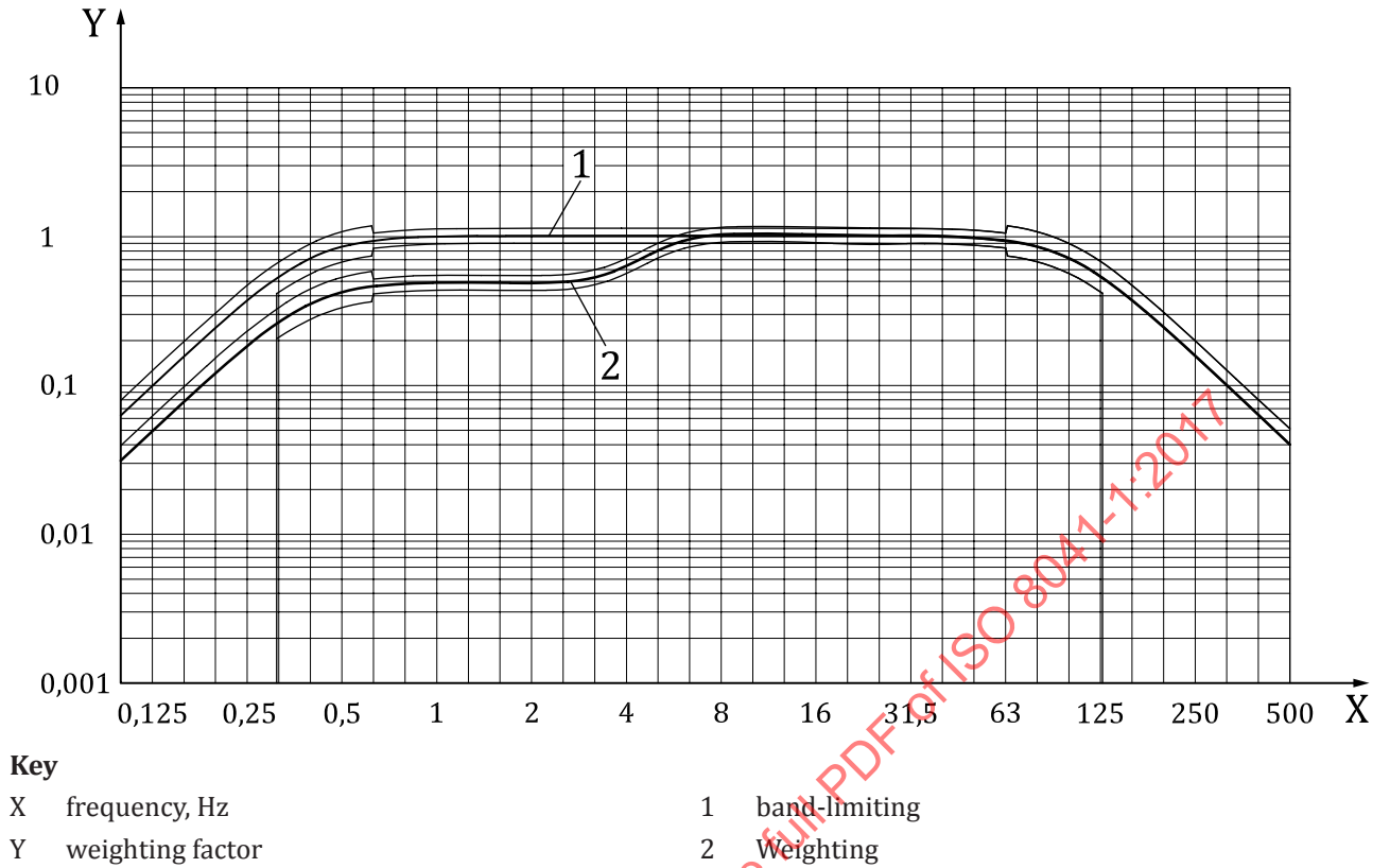
Figure B.13 — Magnitude of frequency weighting W_j for vertical head vibration, x-axis recumbent person, based on ISO 2631-1
