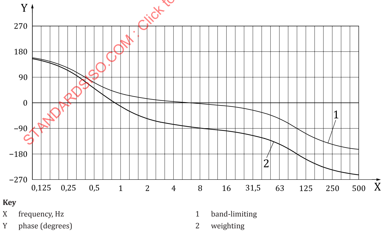
Figure B.8 — Phase of frequency weighting W_e for rotational whole-body vibration, all directions, seated person, based on ISO 2631-1
