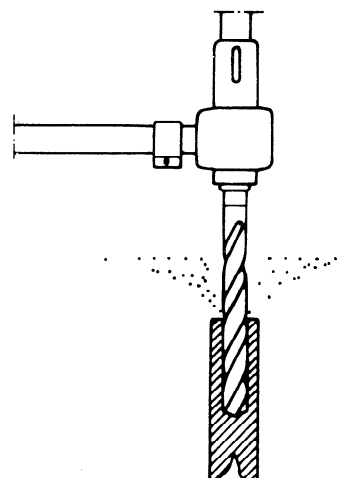
Figure C.2 — Oil-hole drill
