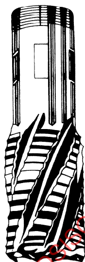
Figure C.3 — Chip-breaking mill cutter
