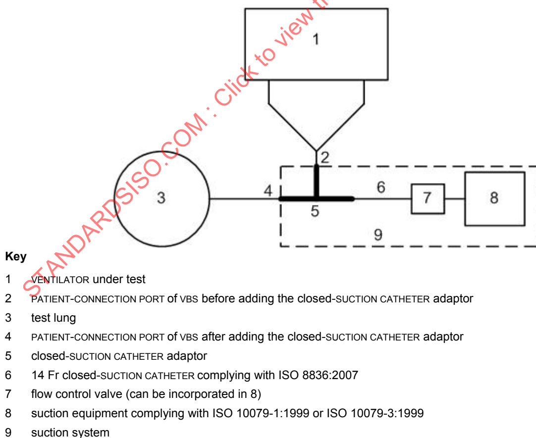
Figure 201.101 — Typical closed-suctioning test setup
