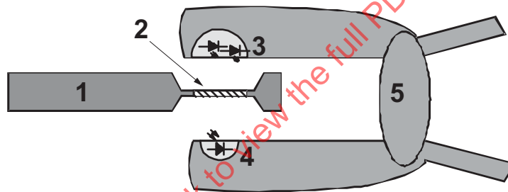
Figure FF.3 — Interface of a FUNCTIONAL TESTER that uses a dye mixture
