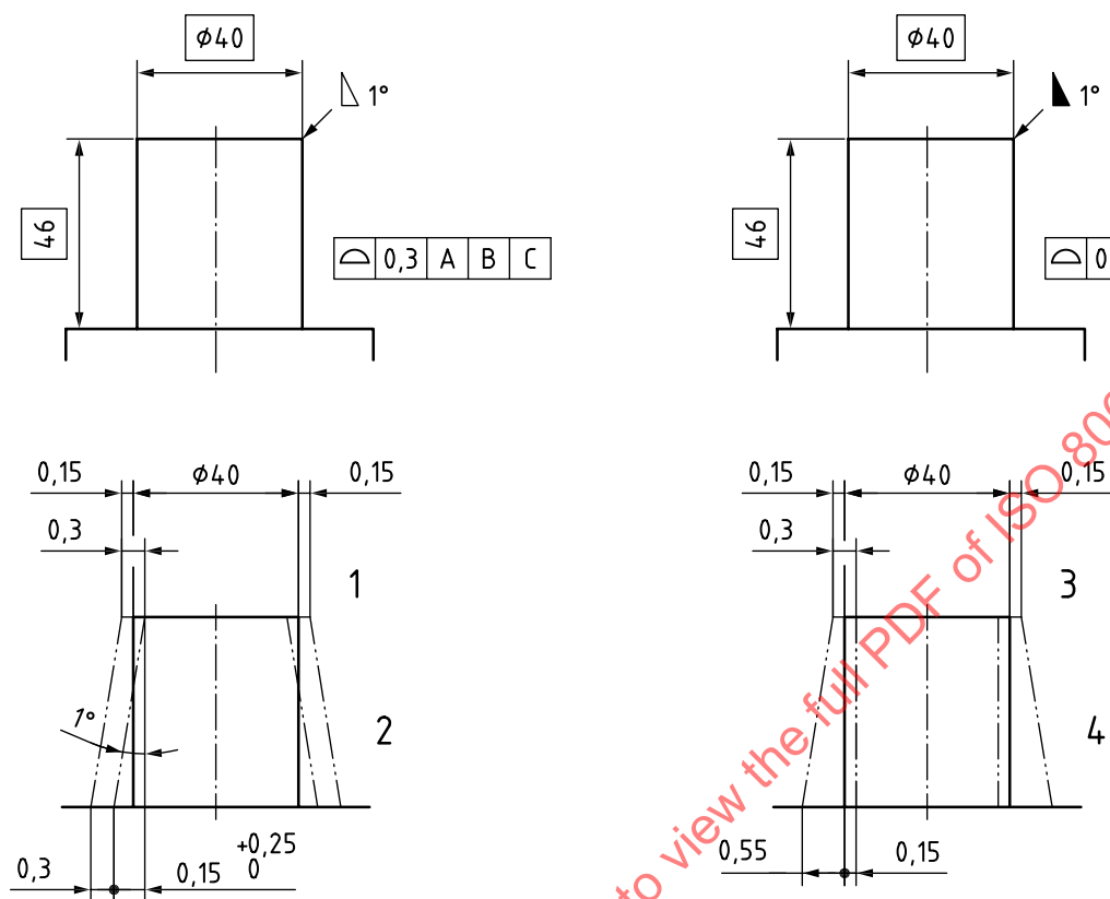
a) Draft angle increasing the ideal model feature(s)
