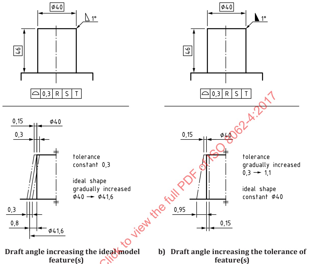
Figure 3 — Draft angles
