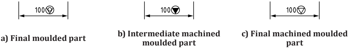
Figure 10 — Examples of nominal dimensions
