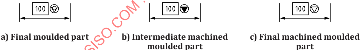
Figure 12 — Examples of TEDs
