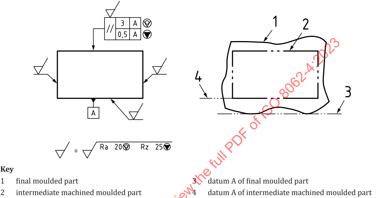
Figure 14 — Example of a datum indication in different part conditions with different datums
