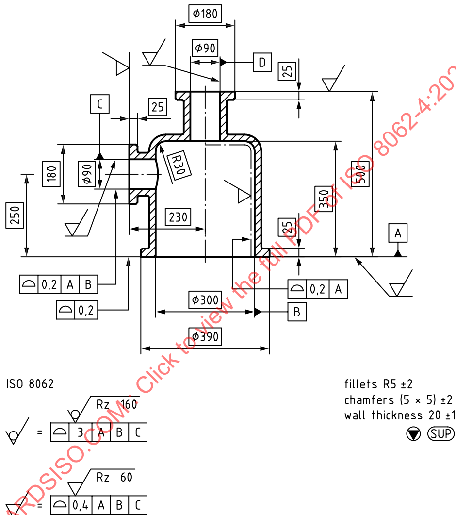
Figure D.3 — Intermediate machined moulded part SUP, particular general tolerances for moulded surfaces
