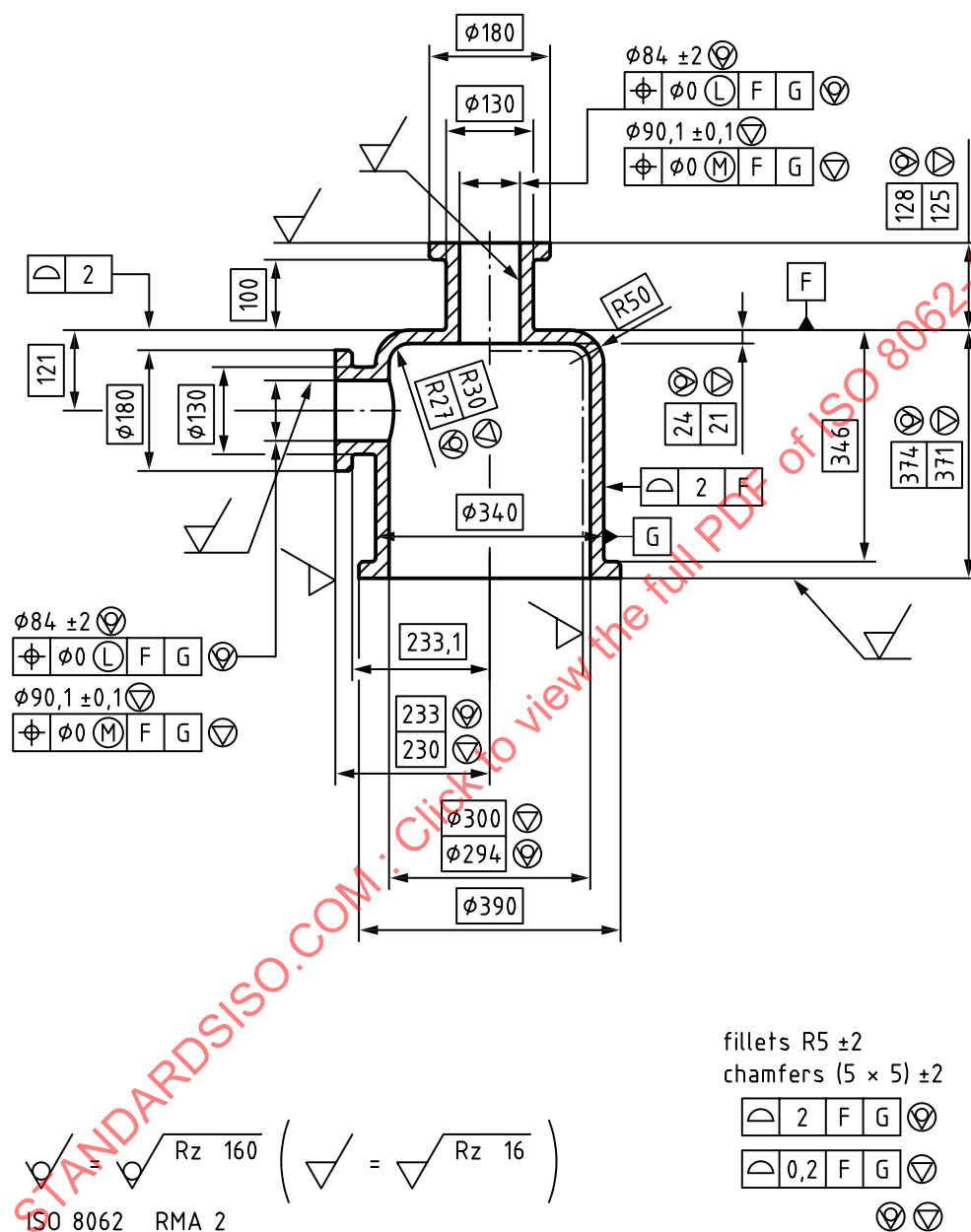
Figure D.4 — Final moulded part and final machined moulded part, multiple tolerancing method
