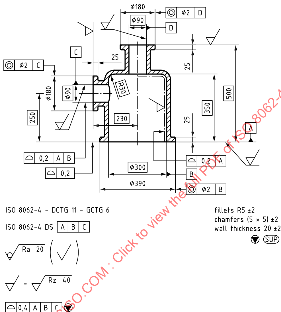
Figure D.2 — Intermediate machined moulded part SUP, general tolerances ISO 8062-3 for moulded surfaces
