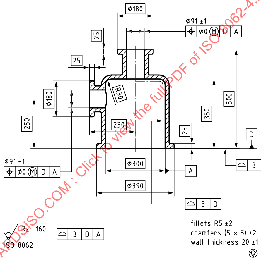
Figure D.1 — Final moulded part, particular general tolerances and individual tolerances
