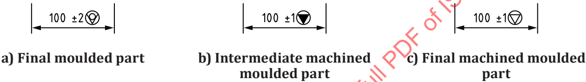
Figure 11 — Examples of nominal dimensions with individual tolerances
