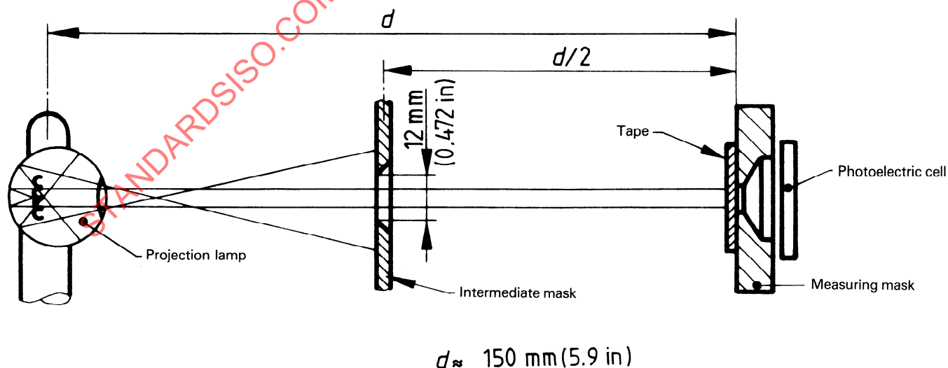
Figure 11 — Measuring device
