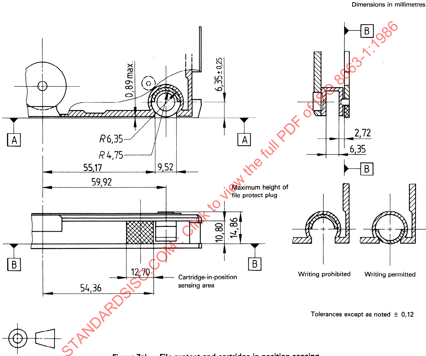
Figure 7a) — File protect and cartridge-in-position sensing
