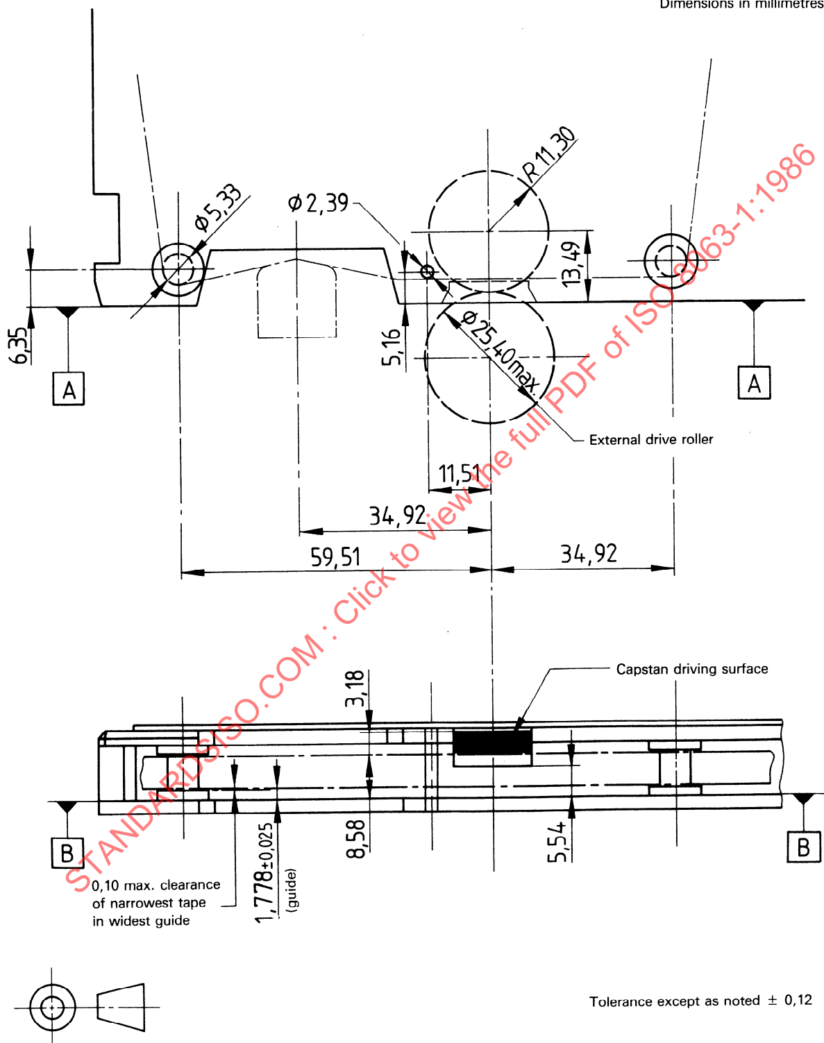
Figure 10a) — Tape path and drive dimensions
