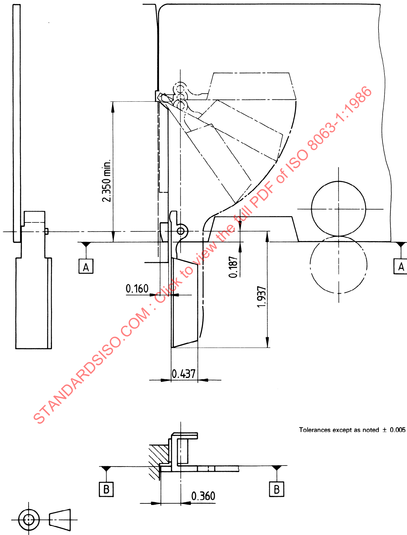
Figure 8b) — Cartridge door profile
