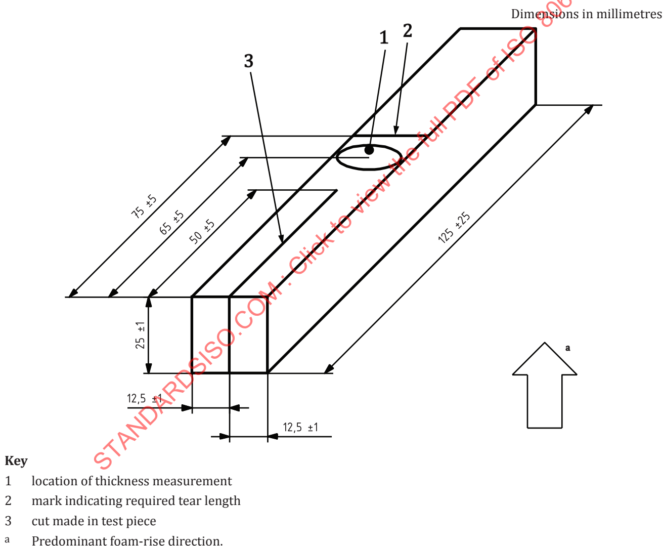
Figure 1 — Trouser test piece
