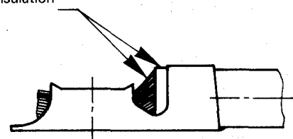
Figure 7 — Conductor and insulation crimp
