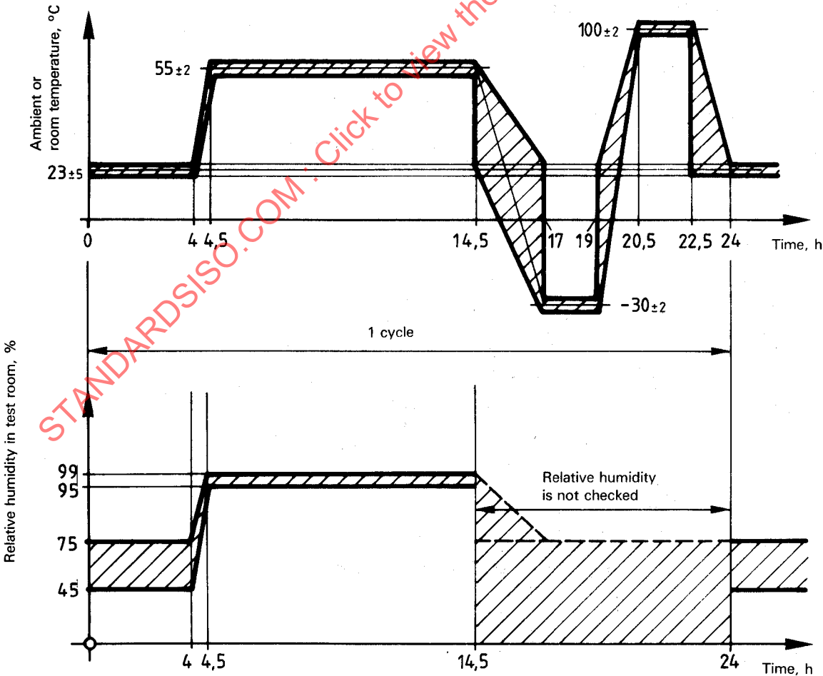
Figure 5 — Temperature and relative humidity cycling test
