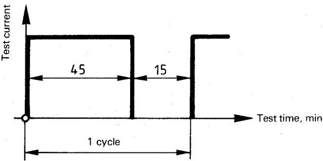
Figure 4 — Current cycling test
