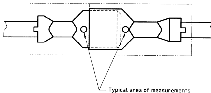
Figure 14 — Test sample for temperature rise test
