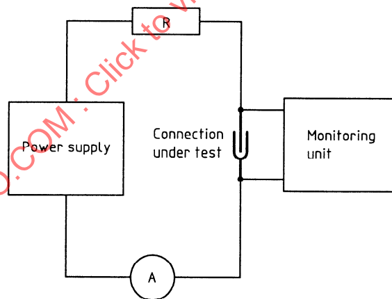
Figure 12 — Connection resistance monitoring at vibration test
