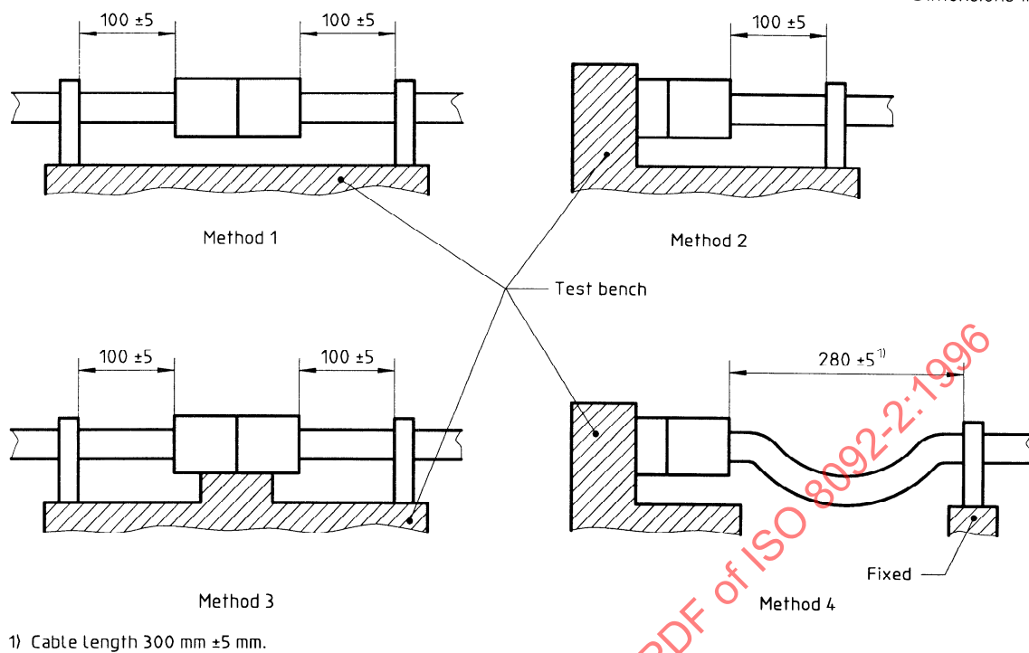
Figure 11 — Vibration test mounting methods
