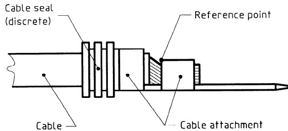
Figure 1 — Male contact
