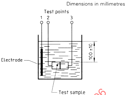
Figure 8 — Watertightness test
