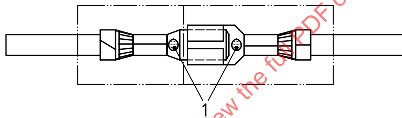
Figure 16 — Test sample for temperature rise test
