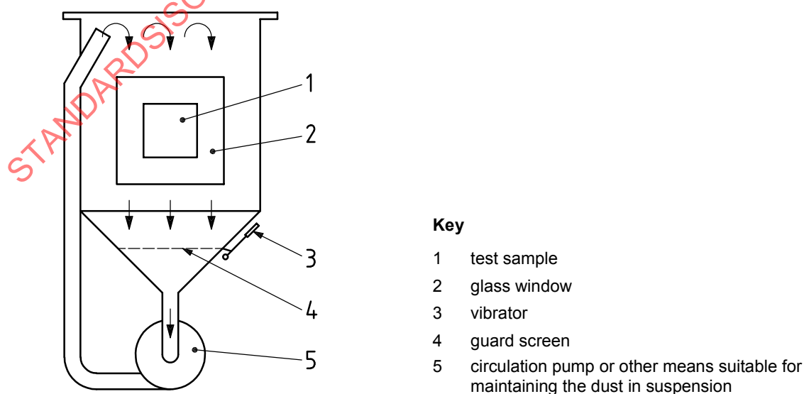
Figure 16 — Dust test
