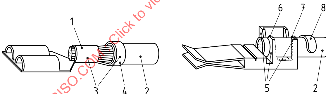
Figure 2 — Male contact
