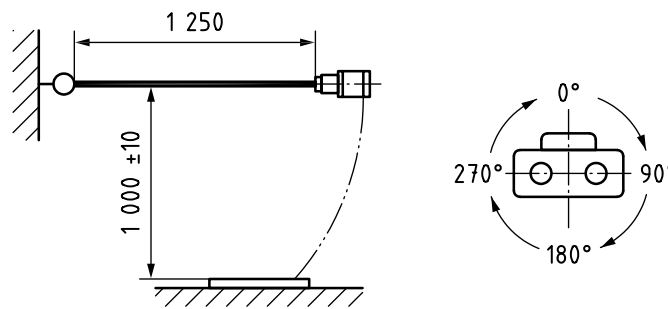
Figure 15 — Drop test arrangement and four orientations to test
