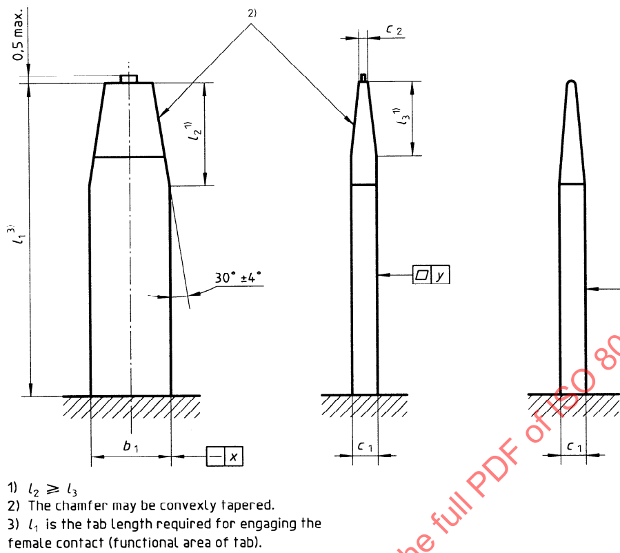
Figure 1 — Tab dimensions
