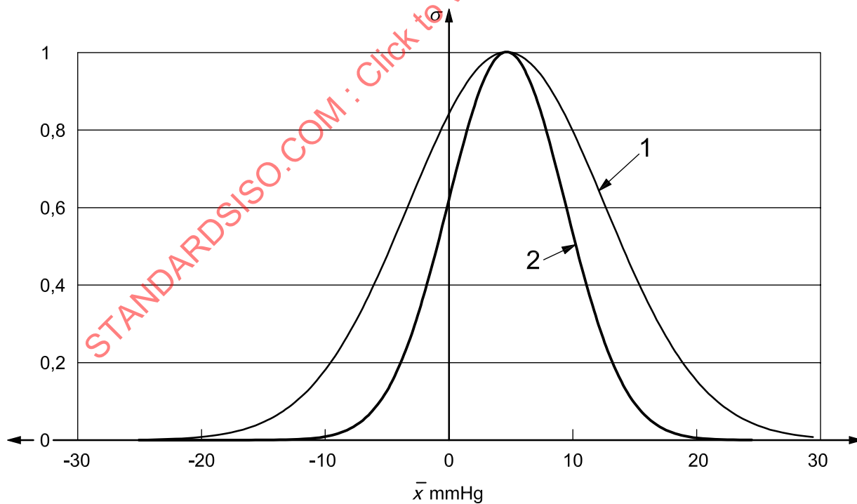
Figure A.1 — Allowable standard deviation for each criterion when the mean error is zero
