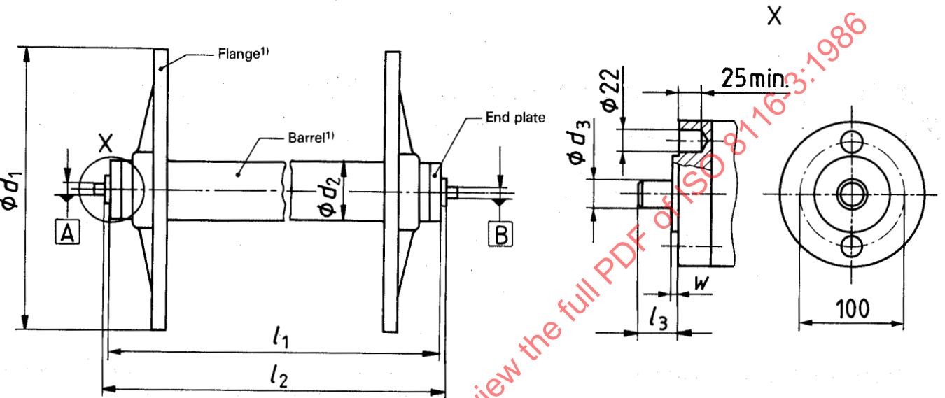
Figure 1 — Weaver's beam with shafts — Type A
